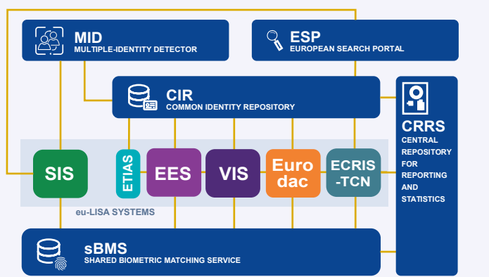
Figure 2. Overview of the Interoperability framework developed by eu-LISA
